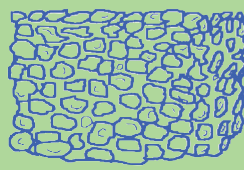
Granular Structure Roundish soil peds that are usually less than 5.0 cm in diameter and look like cookie crumbs
